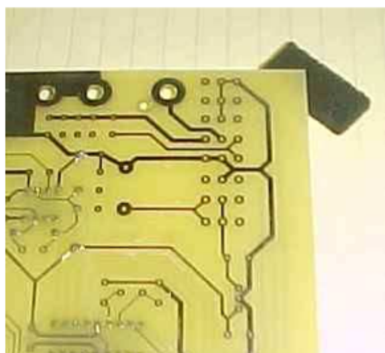
When soldering the sockets, support the corner Using the black foam the ICs are shipped on.
