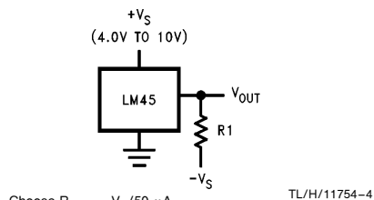
Choose R_1 = -V_S/50\ \mu\text{A} V_{OUT} = (10\ \text{mV}/^\circ\text{C} \times \text{Temp } ^\circ\text{C}) V_{OUT} = +1,000\ \text{mV} at +100^\circ\text{C} = +250\ \text{mV} at +25^\circ\text{C} = -200\ \text{mV} at -20^\circ\text{C} FIGURE 2. Full-Range Centigrade Temperature Sensor ( -20^\circ\text{C} to +100^\circ\text{C} )
