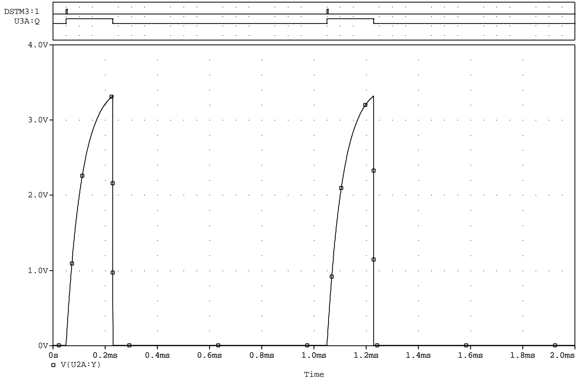
(A) OneShotQ...Input Pulse Shorter than Output
