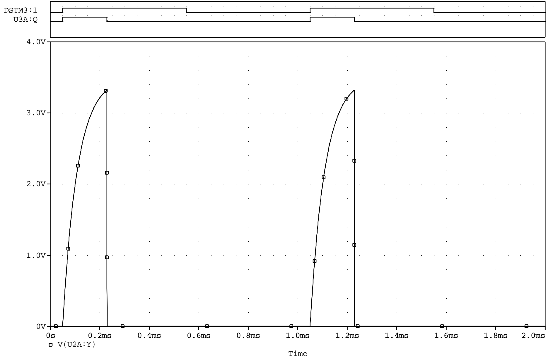
(A) OneShotQ...Input Pulse Longer than Output
