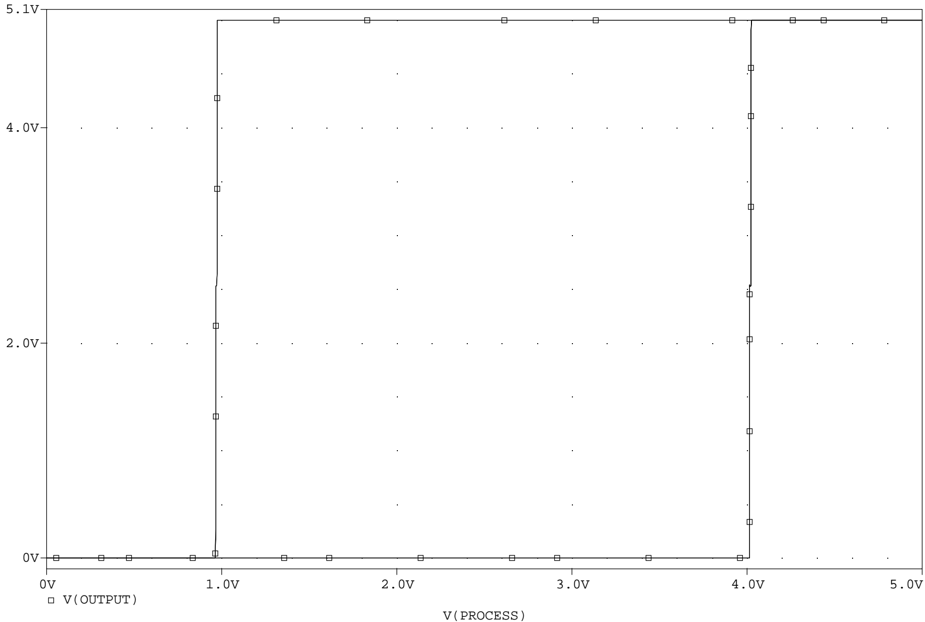
NoiseBlank-HYS....Hysteresis Reflected to Node "PROCESS"
