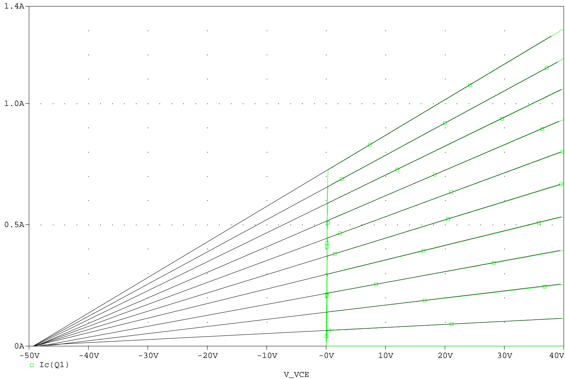
(A) NPN-Sweep with Early Extrapolations Drawn In (2N3055)
