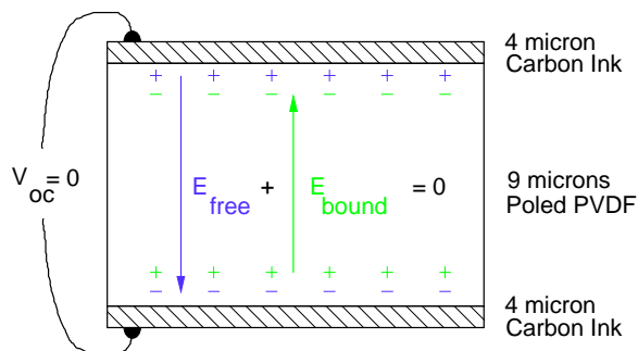
Figure 2: Pyroelectric Detection: Frozen-in field E_{\text{bound}}
